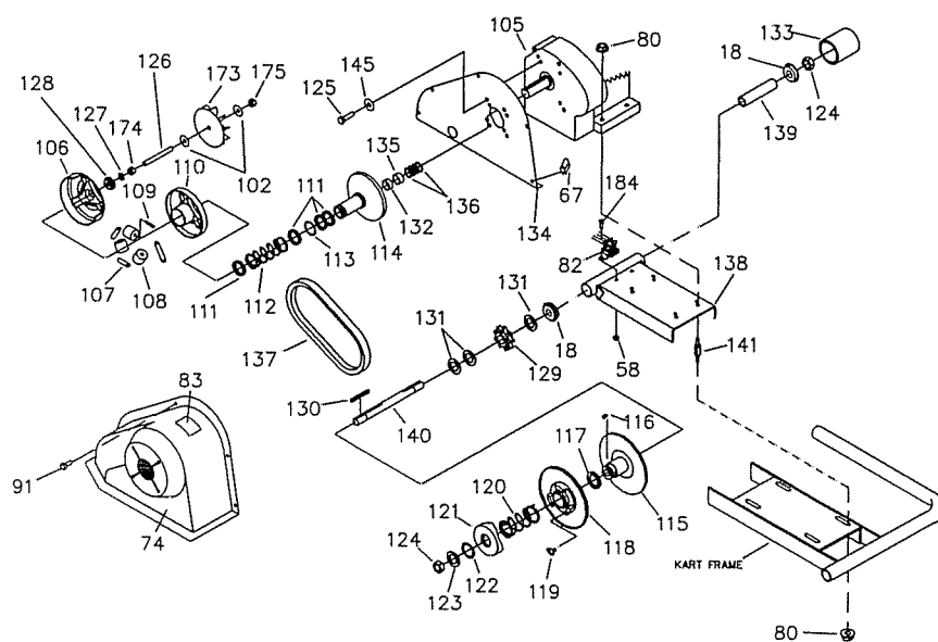
ENGINE MOUNTING DETAIL
