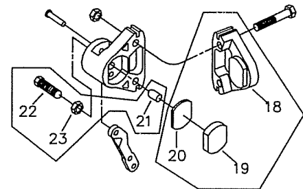
CALIPER BREAKDOWN
